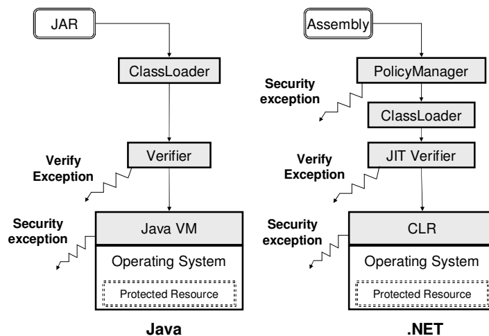
Figure 2. Architecture Overview
