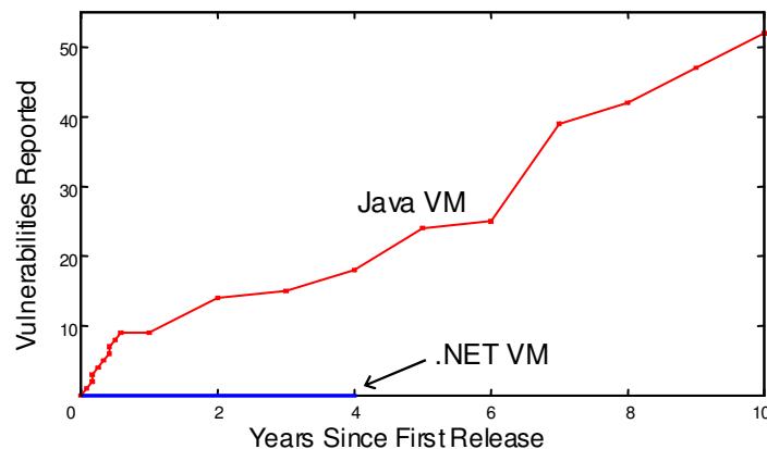
Figure 1. Major security vulnerabilities reported. The value plotted is the cumulative number of security vulnerabilities reported in each platform since the first official release (Java 1.0 in January 1996 [40]; .NET 1.0 in January 2002 [26]).
