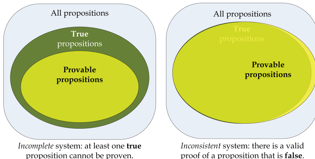
Figure 12.1. Incomplete and inconsistent axiomatic systems.
