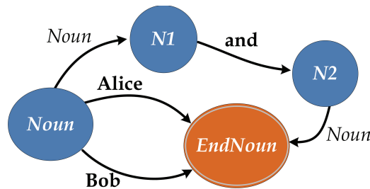
Figure 2.4. Alternate Noun subnetwork.
