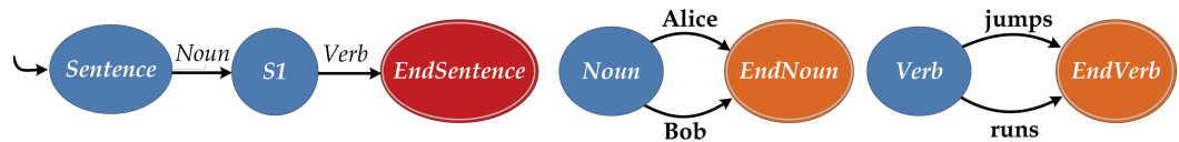
Figure 2.3. Recursive transition network with subnetworks.
