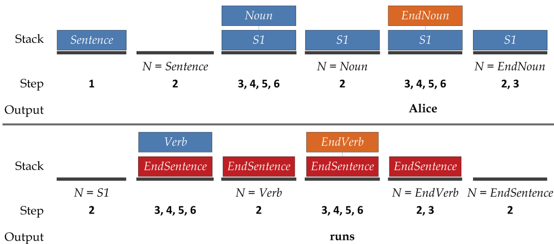
Figure 2.5. RTN generating “Alice runs”.
