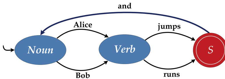
Figure 2.2. RTN with a cycle.
