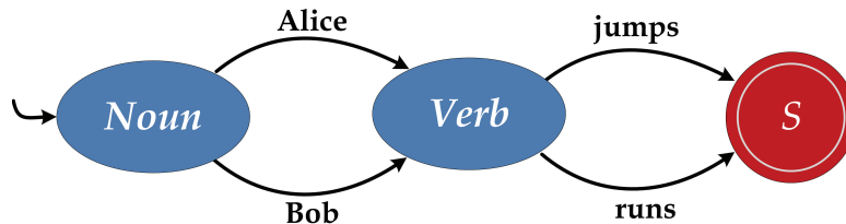
Figure 2.1. Simple recursive transition network.
