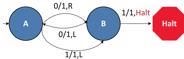
Figure 12.3. Two-state Busy Beaver Machine.
