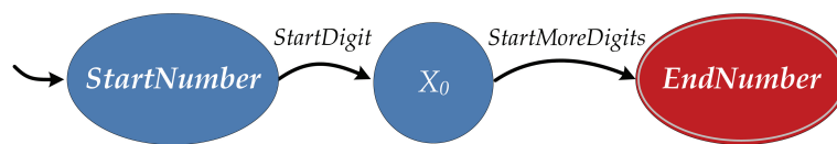
Figure 2.7. Converting the Number productions to an RTN.
