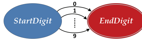
Figure 2.9. Converting the Digit productions to an RTN.
