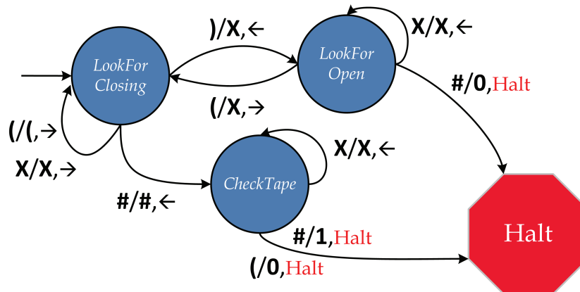
Figure 6.8. Checking parentheses Turing Machine.
