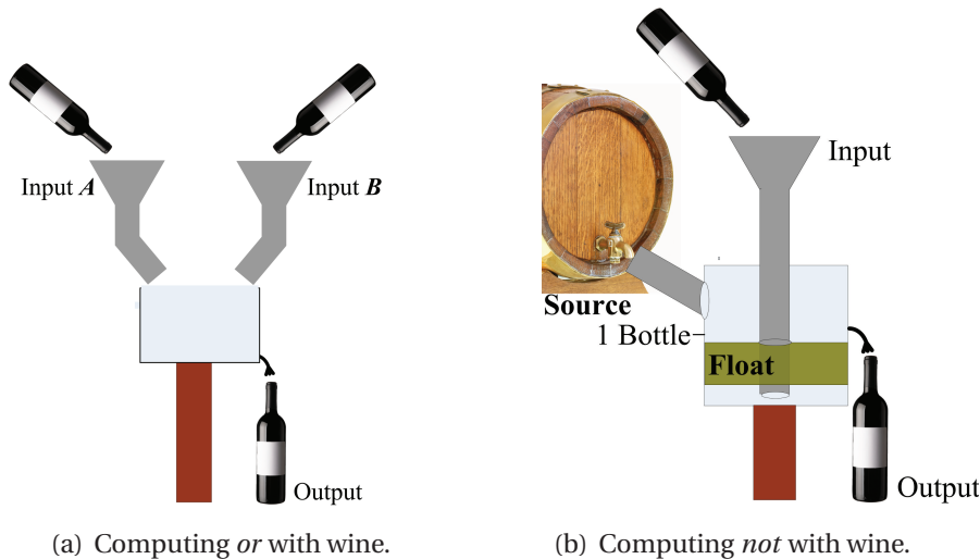
Figure 6.2. Computing logical or and not with wine
