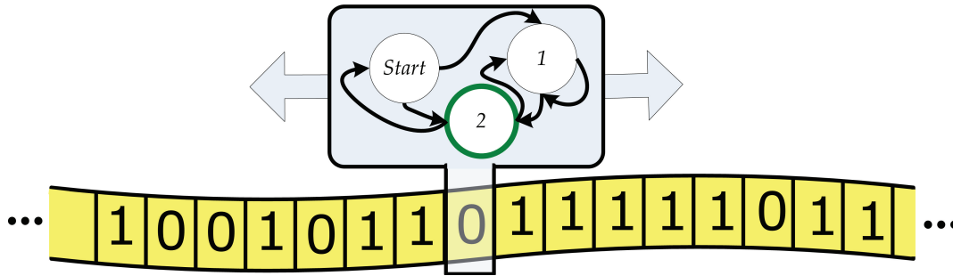
Figure 6.6. Turing Machine model.
