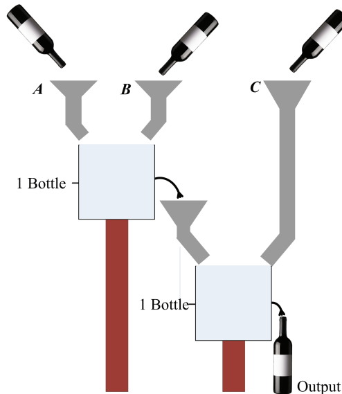
Figure 6.3. Computing and3 by composing two and functions.
