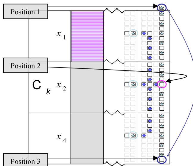
Figure 8: Finalization Tile.
