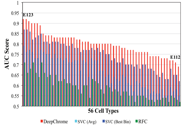
Fig. 3: Performance Evaluation on Test Set. (Best viewed in color) The bar graph represents AUC scores of DeepChrome versus state-of-the-art baseline models for 56 cell types (i.e. 56 different classification tasks). The results have been arranged from best performing cell type (E123) to the worst performing cell type (E112) for the test set (6600 genes). DeepChrome (Average AUC = 0.80) consistently outperforms both SVM (Average AUC: SVM Best Bin = 0.75 and SVM Avg = 0.66) and Random Forest Classifier (Average AUC = 0.59) for the task of binary classification of gene expression. SVM based baseline has a separate model for each bin (bin specific model), thus, results for both average AUC scores across all bins (SVM Avg) and best performing AUC score among the bins (SVM Best Bin) are presented.
