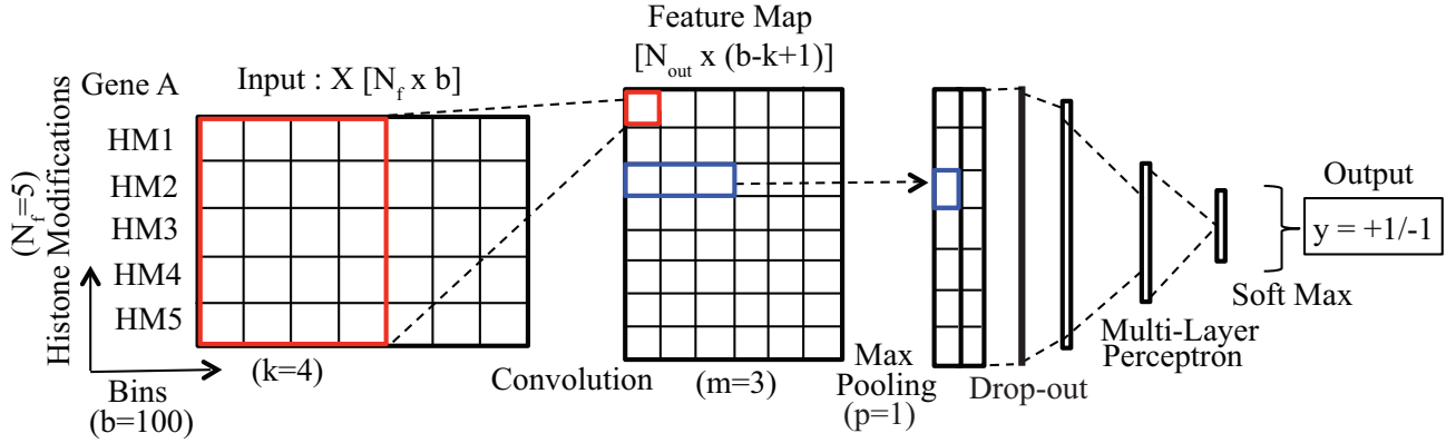
Fig. 2: DeepChrome convolution neural network (CNN) model. The input matrix X , comprising of 100 bins with signals from five histone modifications, goes through different CNN stages. These stages are : convolution, pooling followed by dropout, and multi-layer perceptron with alternating linear and non-linear layers. Softmax function, in the end, maps the output from the model into classification prediction.
