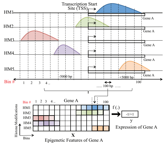
Fig. 1: Feature Generation for DeepChrome model. Bins of length 100 base-pairs (bp) are selected from regions ( \pm 5000 bp) flanking the transcription start site (TSS) of each gene. The signal value of all five selected histone modifications in bins forms input matrix X , while discretized gene expression (label +1/-1 ) is the output y .
