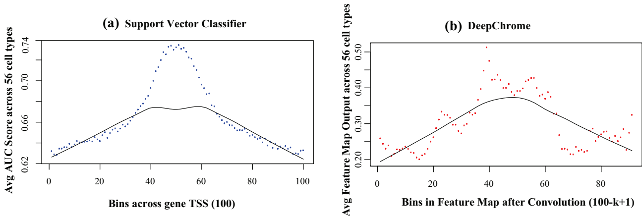
Fig. 4: Validating the influence of positions for gene expression classification. Cheng et al. (2011) reported that the bin positions closer to the transcription start site (TSS) of each gene are more important when predicting gene expression. This is confirmed by our implementation of this bin-specific baseline model in (a). For each bin position, it shows the mean AUC score across all the cell types. In (b) we plot the filter outputs from the convolution layer of DeepChrome model. For each bin, its value has been averaged across all filters and cell-types. The solid lines represent the best-curve fit to the data points plotted in the figures. The trends for both (a) and (b) are similar.
