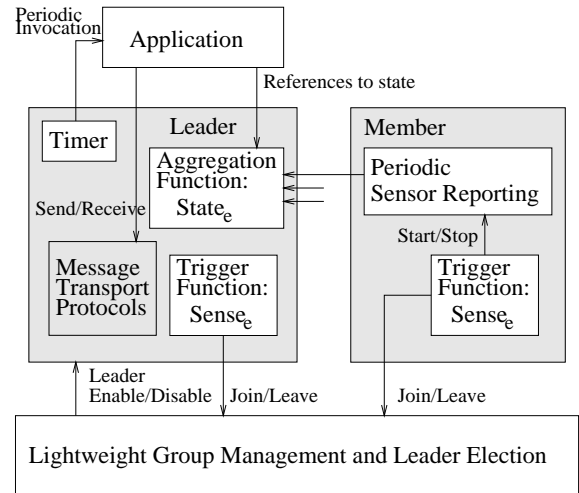
Figure 2. Middleware Architecture
