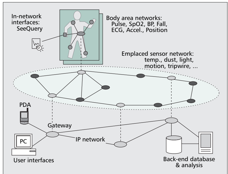
Figure 1. AlarmNet architecture.
