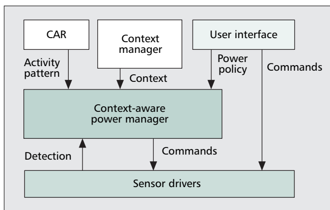
■ Figure 5. CAPM components in AlarmNet.
