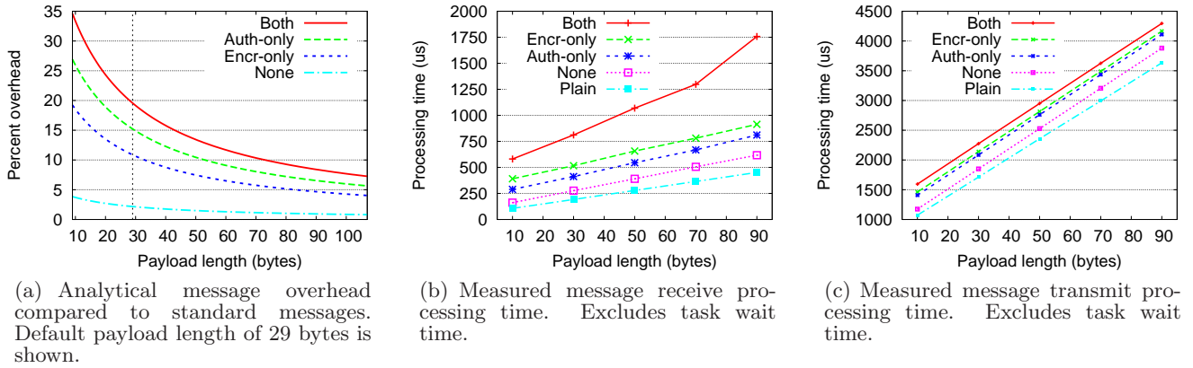
Figure 3: AMSecure overhead and performance for varying payload lengths up to 802.15.4 maximum.
