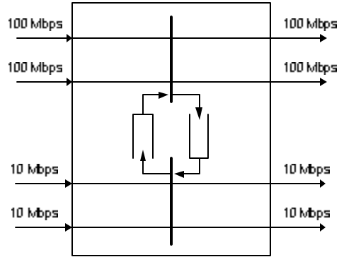
Dual-Speed Ethernet Hub
