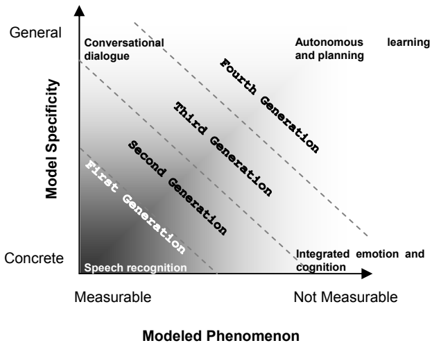
Figure 2 - Generation Framework for HBR
