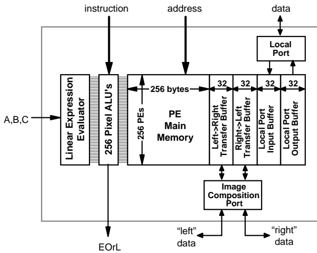
Figure 5: Block diagram of Enhanced Memory Chip.
