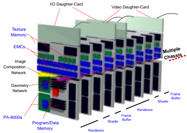
Figure 3: One-chassis PixelFlow system.
