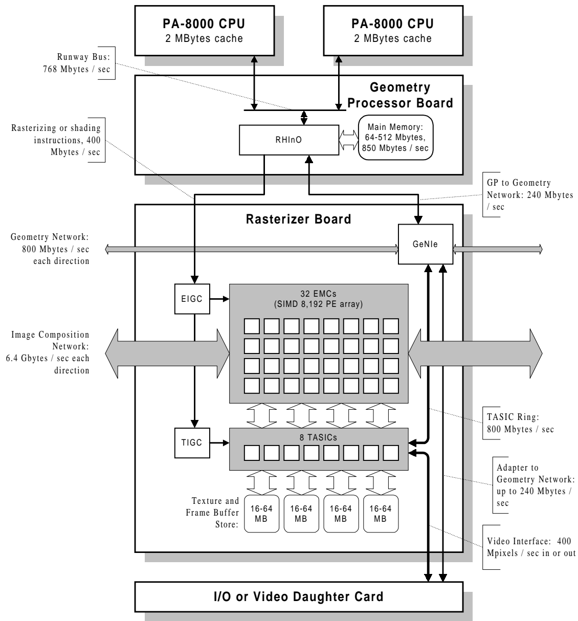
Figure 4: PixelFlow Flow Unit with CPUs and IO/Video adapter.
