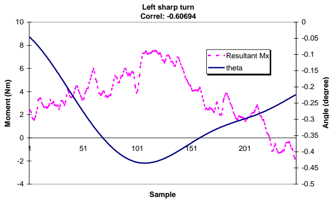
Figure 9. Overall walker turning moment M_x vs. \theta
