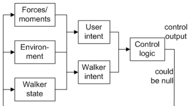
Figure 1. Walker Control System Architecture
