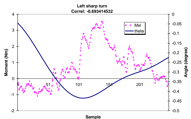
Figure 8. Turning moment in left handle M_{XL} vs. \theta
