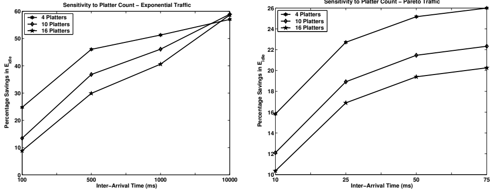
Figure 7: Sensitivity to Number of Platters in the Disk Assembly
