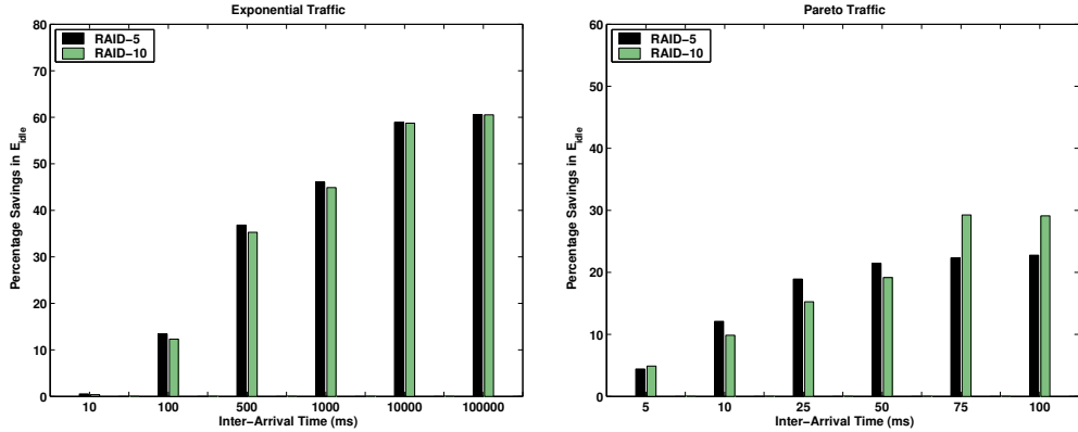
Figure 10: Sensitivity of DRPM_{perf} to RAID-Level.
