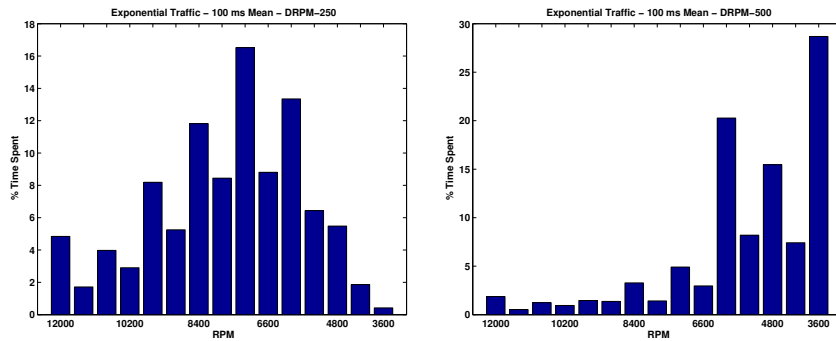
Figure 14: Average Residence-Times in the Different RPMs for the DRPM Heuristic for n = 250, 500 . The values presented have been averaged over all the disks in the array. A step-size of 600 RPM is used. Note that the lower RPMs are exercised more with a larger n .
