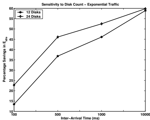
Figure 11: Sensitivity to Number of Disks in the Array
