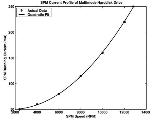
Figure 2: Current Drawn by Sony Multimode Hard Disk
