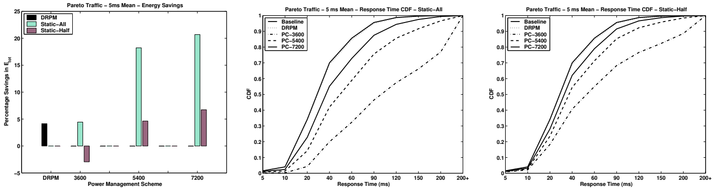
Figure 15: Static RPM vs. DRPM. The workload is \langle \text{Par}, 5 \rangle and the graphs are presented for the quadratic power model. For DRPM, we chose n = 1000 .
