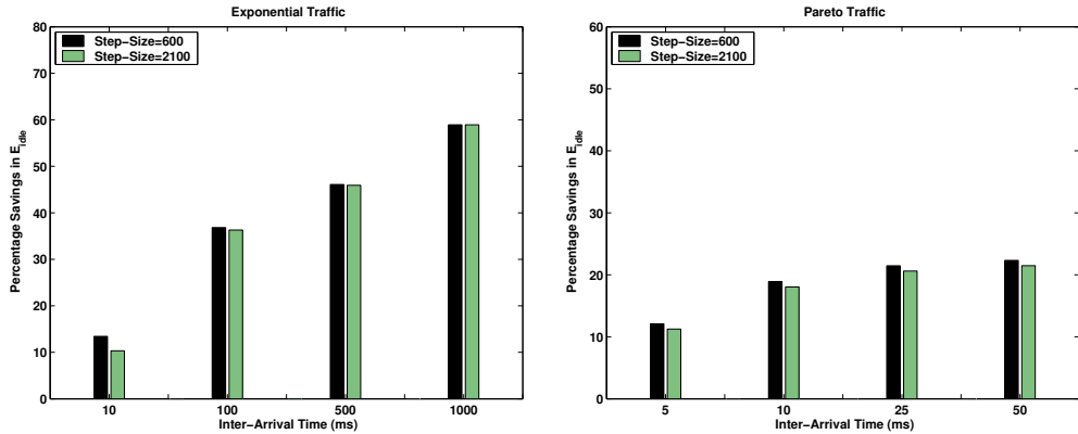
Figure 8: Sensitivity to the Step-Size Used by DRPM
