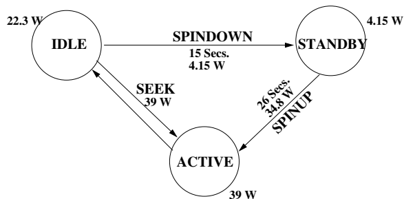
Figure 4: TPM Power Modes
