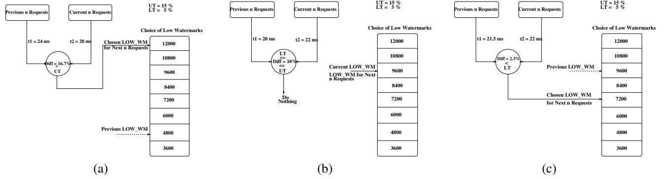
Figure 12: The operation of the DRPM heuristic for UT = 15\% and LT = 5\% . In each figure, for the choice of low watermarks, the dotted line shows where LOW\_WM is before the heuristic is applied and the solid line shows the result of applying the scheme. The percentage difference in the response times, t_1 and t_2 between successive n -request windows, diff , is calculated. (a) If diff > UT , then LOW\_WM is set to the maximum RPM for the next n requests. (b) If diff lies between the two tolerance-limits, the current value of LOW\_WM is retained. (c) If diff < LT , then the value of LOW\_WM is set to a value less than the maximum RPM. Since diff is higher than 50% of LT but lesser than 75% of LT in this example, it is set two levels lower than the previous LOW\_WM . If it was between 75% and 87.5%, it would have been set three levels lower, and so on.
