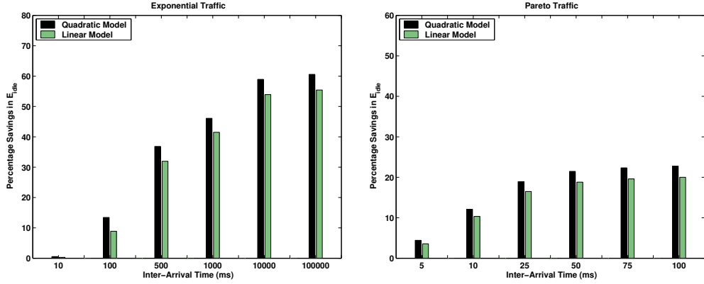
Figure 9: Behavior of DRPM_{perf} for a Power Model that relates the RPM and P_{idle} linearly
