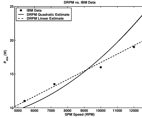
Figure 3: Comparison of DRPM Model to IBM Projections given in [40]
