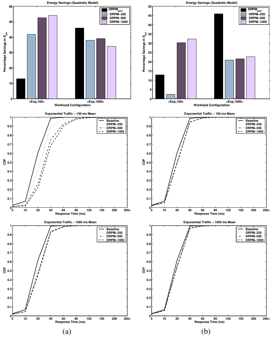
Figure 16: Controlling UT and LT for Power-Performance Tradeoffs. (a) presents the results for UT=15%,LT=10%. (b) presents the results for UT=8%,LT=5%.
