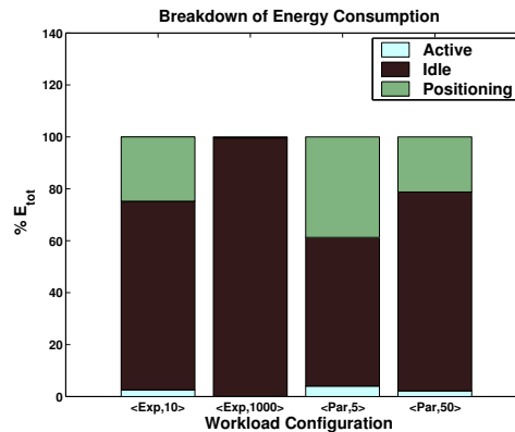
Figure 5: Breakdown of E_{tot} for the different workloads. On the x-axis, each pair represents a workload defined by <Probability Distribution, Mean Inter-Arrival Time> pair.
