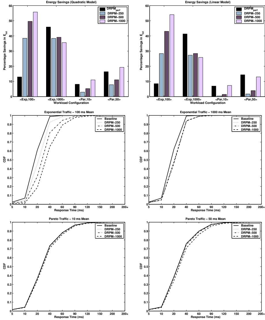
Figure 13: DRPM Heuristic Scheme Results. UT = 15\% , LT = 5\% , N_{min} = 0 . The results are presented for n = 250, 500, 1000 , referred to as DRPM-250, DRPM-500, and DRPM-1000 respectively.
