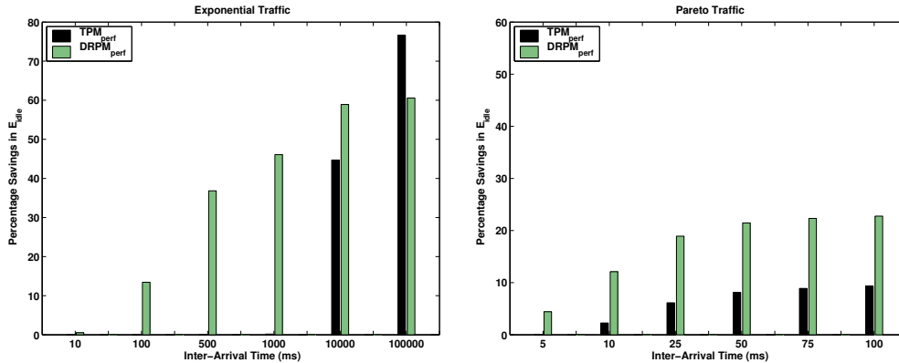
Figure 6: Savings in Idle Energy using TPM_{perf} and DRPM_{perf} are presented for the quadratic power model.
