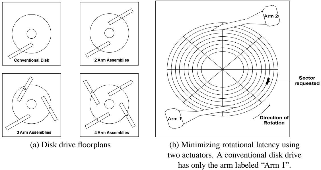
Figure 4.4: Intra-disk parallelism along the A -dimension.
