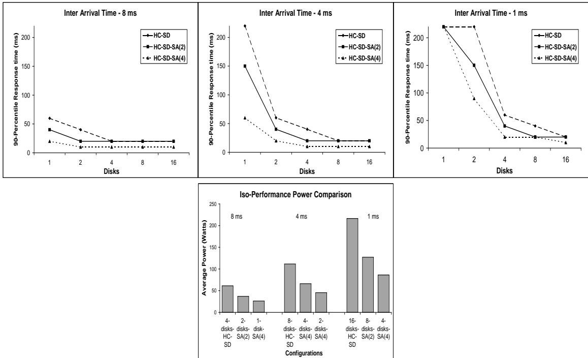
Figure 4.8: Performance and power characteristics of RAID arrays using intra-disk parallel drives
