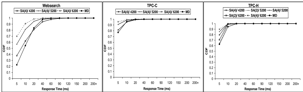
Figure 4.7: Performance of reduced RPM HC-SD-SA(n) designs whose response times match or exceed MD . Each legend entry is in the format: \langle HC-SD-SA(n) \text{ configuration} \rangle / \langle RPM \text{ Value} \rangle .
