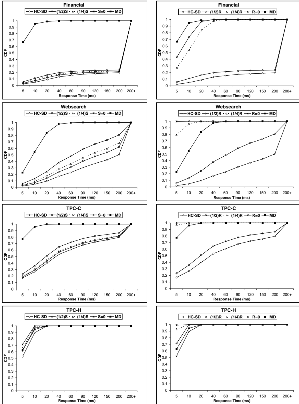
Figure 4.3: Bottleneck analysis of HC-SD performance. The graphs on the left column show the effect of seek time and the ones in the right column show the impact of rotational latency.
