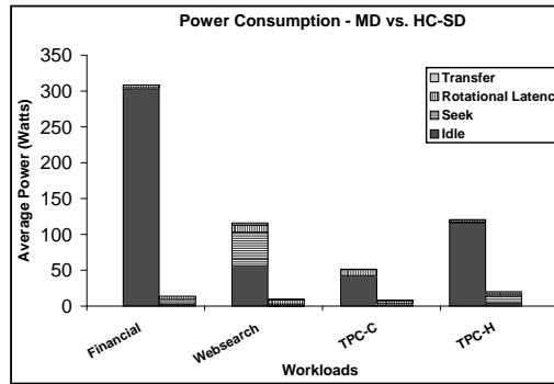
Figure 4.2: The power gap between MD and HC-SD . For each workload, the bar on the left corresponds to MD and the one on the right to HC-SD .
