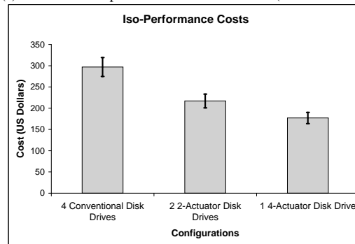
(b) Iso-performance cost comparison between conventional and intra-disk parallel drives. The error-bars give the cost range based on the values in the table on the left.
