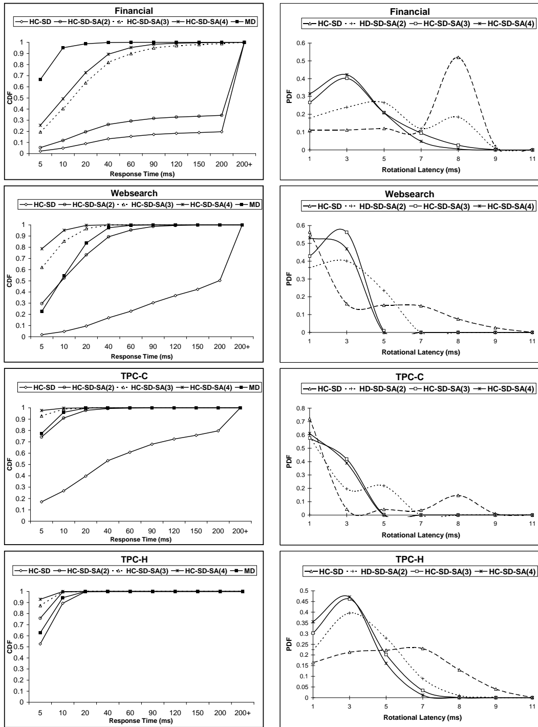
Figure 4.5: Performance impact of the HC-SD-SA(n) design.
