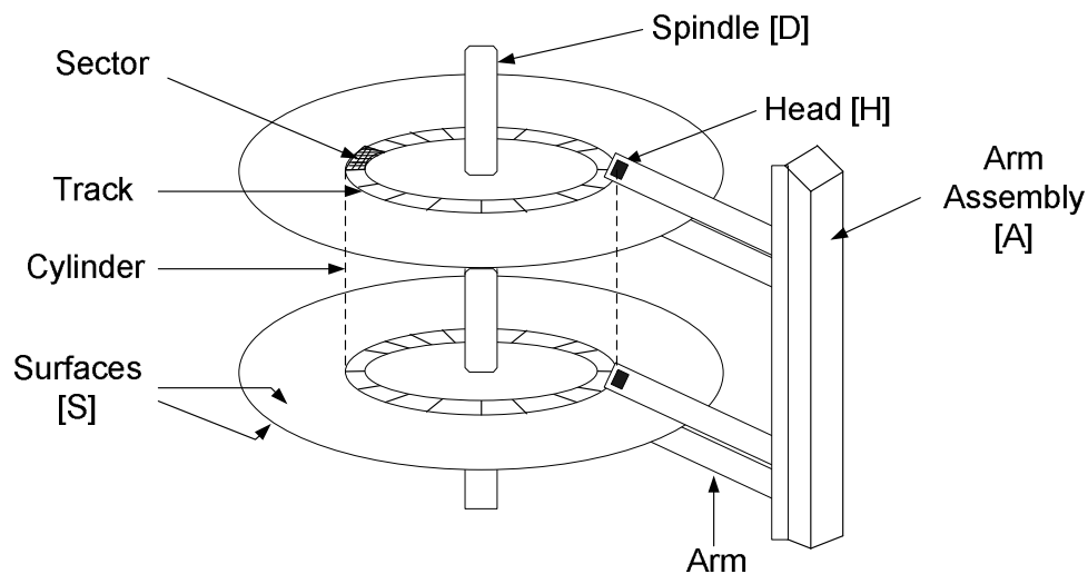
Figure 1.1: Hard Disk Drive Architecture. The various locations where parallelism can be incorporated are indicated within square-brackets.
