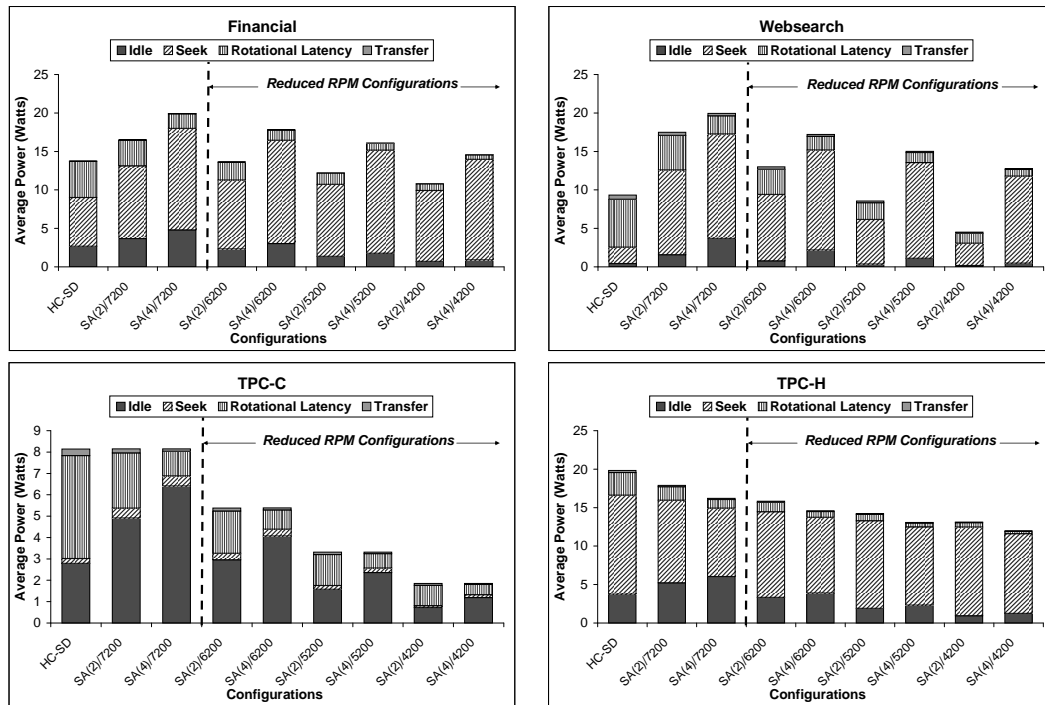
Figure 4.6: Average power consumption of the disk drive configurations. Each bar corresponds to a particular disk drive configuration and the x-axis labels are in the format: \langle HC-SD-SA(n) \text{ configuration} \rangle / \langle RPM \text{ Value} \rangle .
