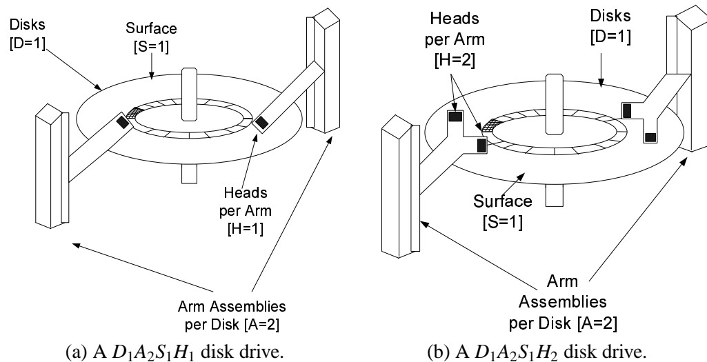
Figure 3.1: Example design points within the DASH intra-disk parallelism taxonomy.
