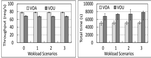
(a) Average throughput. (b) Total time for simulation.
