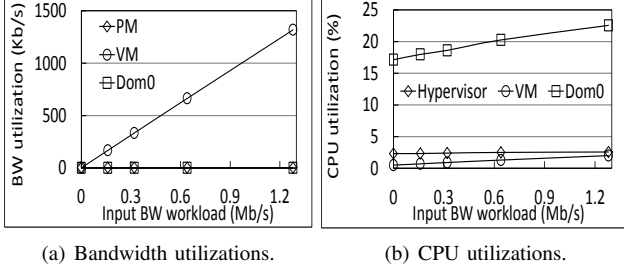
Figure 5. Resource utilizations for intra-PM bandwidth-intensive workload.
