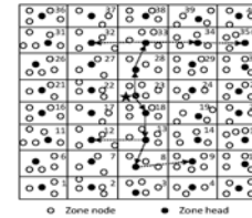
Algorithm overview
