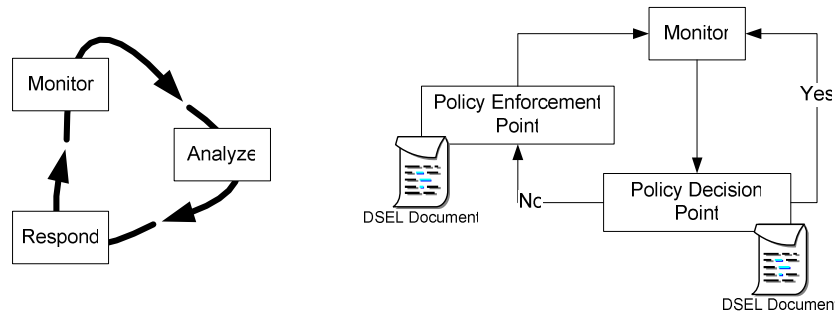
Figure 2: Conceptual model for GDSA. The figure on the left shows the conceptual model as a classic data-driven control loop. The figure on the right shows more detail with the role of DESL as a specification language.
