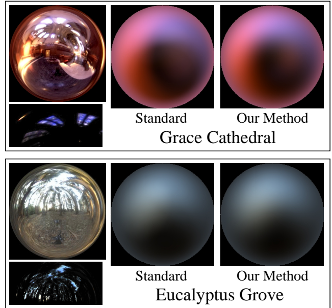
Figure 3: A comparison of irradiance maps from our method to those from standard prefiltering. The irradiance map resolutions are 256x256. For each light probe, the left image is a tone-mapped version of the environment. Below that, we show the brightest parts of the environment on a linear scale. Both environments have bright bluish lights—from stained-glass windows, and the sky respectively—which are not apparent in the tone-mapped images. This accounts for the bluish portions of the irradiance maps. It can be seen that our method produces a result very close to the correct answer. Note that our rendering algorithm does not actually use irradiance maps; we computed them here solely for the purposes of the quality comparison. The coordinate mapping in the images is such that the center of the image is straight forward ( \theta = 0 , the north pole or +Z), the circumference of the image is straight backwards ( \theta = \pi , the south pole or -Z), and \theta varies uniformly in the radial direction from 0 to \pi . The azimuthal angle \phi corresponds to the image polar angle.
