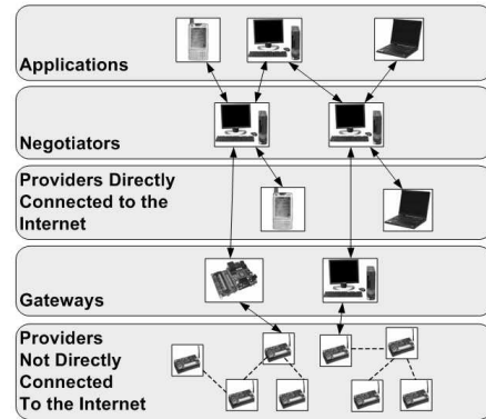
Fig. 1. Physicalnet Architecture.
