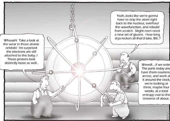
Quantum mechanics.
