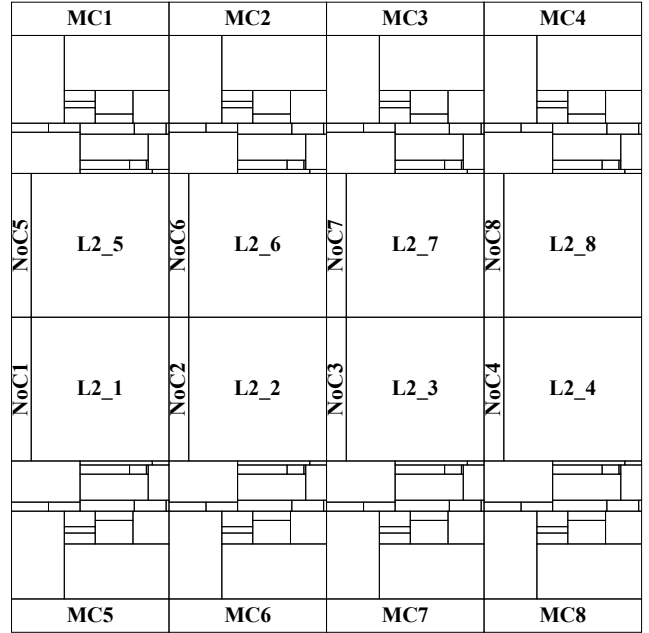
Figure 2. CMP floorplan of 8 Penryn-like cores with L2 cache, NoCs and Memory Controllers added.
