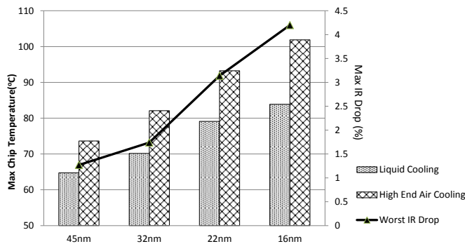
Figure 4. A comparison between chip max temperature and worst IR drop across different technologies
