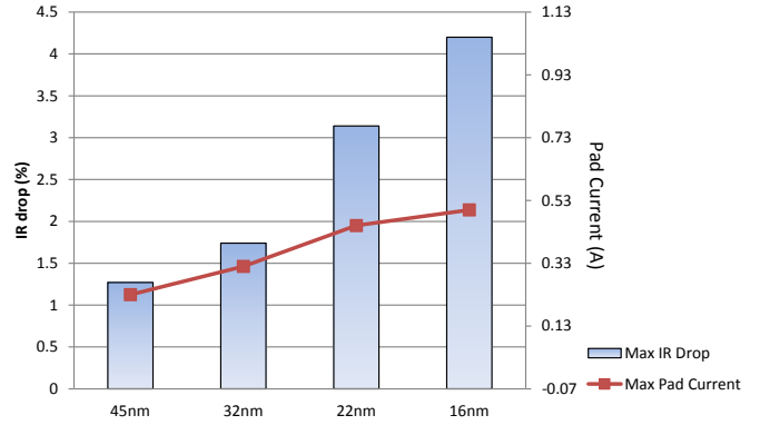
Figure 3. Max pad current and max on-chip IR drop at each technology node. The upper range of the right Y-axis is the threshold current value for EM (at 100°C). For IR drop, we do not set an explicit threshold value but a 3.8% IR drop could cause as high as 51% delay increase [22]. IR drop therefore poses a more significant risk to failure than EM.
