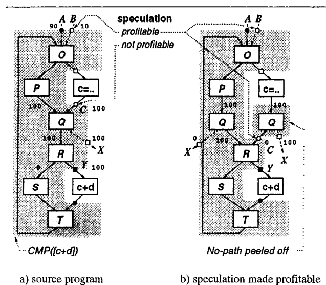
Figure 7: Integrating speculation and restructuring.
