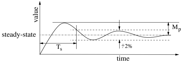
Fig. 1. Definition of settling time ( T_s ) and overshoot ( M_p )
