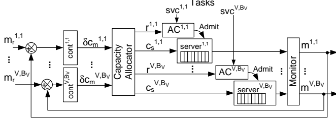
Fig. 2. QoS management architecture using feedback control
