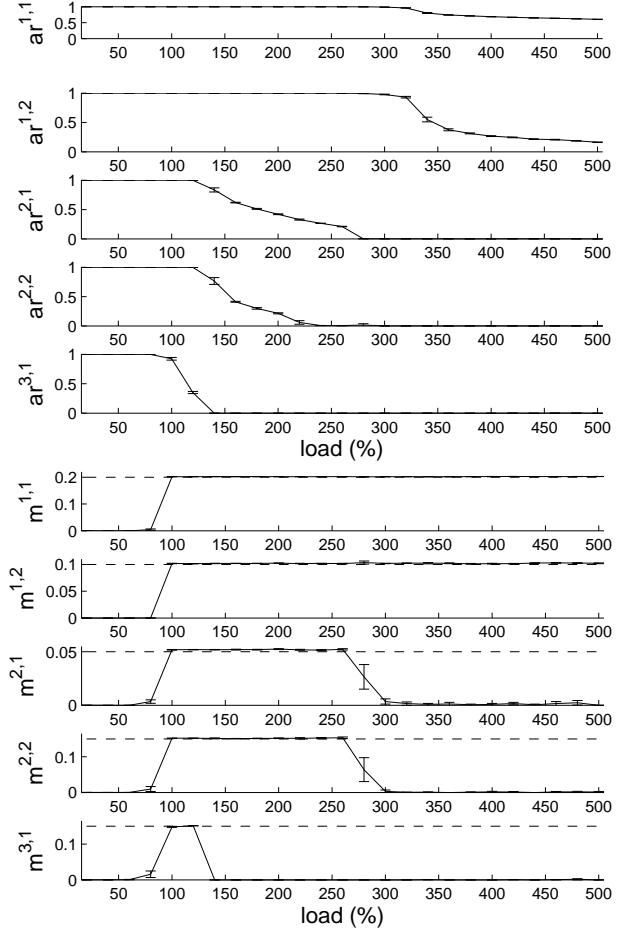
Fig. 5. Experiment 1: Varying load
