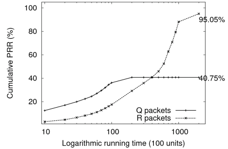
Fig. 2. Comparison of delivery time of Q and R packets.
