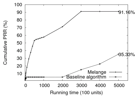
Fig. 3. Cumulative probabilistic distribution function for Performance of Mélange compared to epidemic routing approach.
