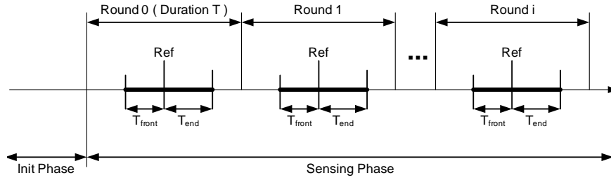
Fig. 1. Node Working Schedule
