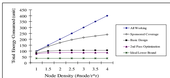
Fig. 11. Total Energy Consumption per Unit of Time
