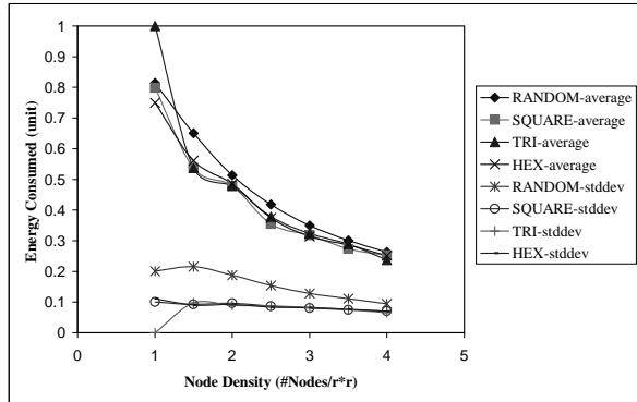
Fig. 16. Energy Consumed for Grid Deployments
