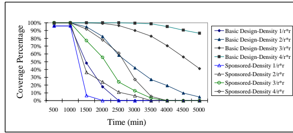
Fig. 14. Sensing Coverage Over Time
