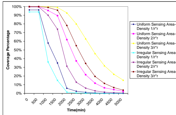
Fig. 34. Sensing Coverage Over Time
