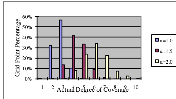
Fig. 20. Actual Degree of Coverage for Differentiated Surveillance
