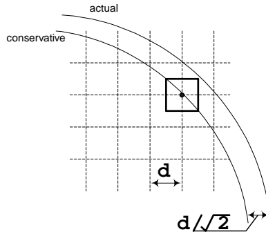
Fig. 5. Grid Size Granularity Issues
