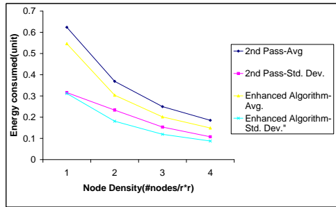
Fig. 22. Single Node Energy Consumption: Average and Standard Deviation(Target Size=2)
