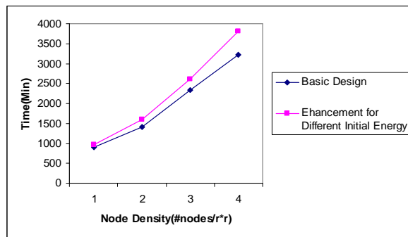
Fig. 30. Half-Life of the Network
