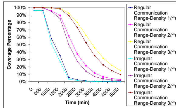
Fig. 36. Sensing Coverage Over Time
