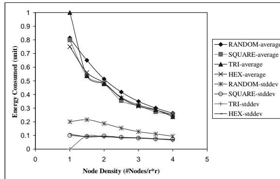
Fig. 16. Energy Consumed for Grid Deployments
