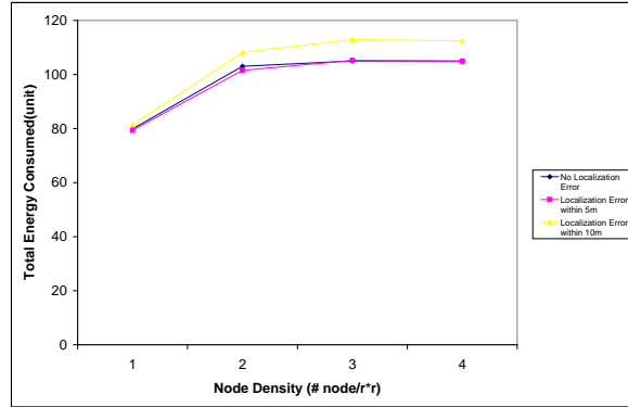
Fig. 31. Total Energy Consumption per Unit of Time
