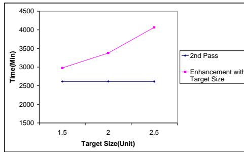
Fig. 25. Half-life of the Network Vs. Target Size (Node Density=2/r*r)
