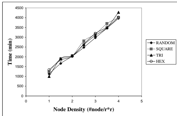
Fig. 17. Half-Life for Grid Deployments
