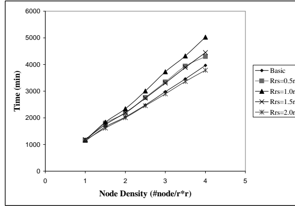
Fig. 28. Half-Life for Reference Point Scattering
