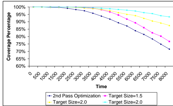
Fig. 26. Sensing coverage over time ( 3/r^*r )
