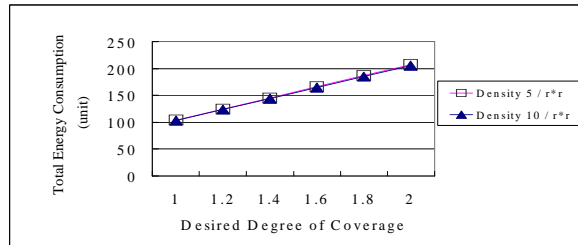
Fig. 19. Total Energy Consumed for Differentiated Surveillance
