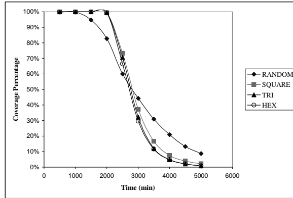
Fig. 18. Coverage Over Time for Grid Deployments
