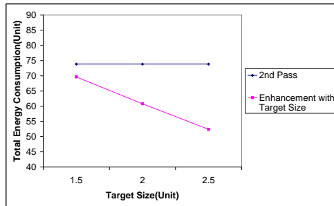
Fig. 23. Total Energy Consumption Vs. Target Size(Node Density=2/r*r)
