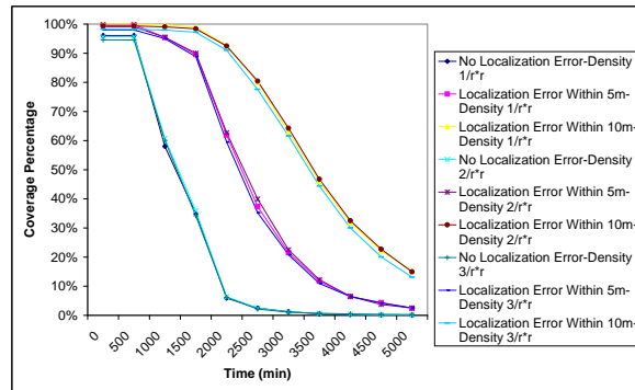
Fig. 32. Sensing Coverage Over Time
