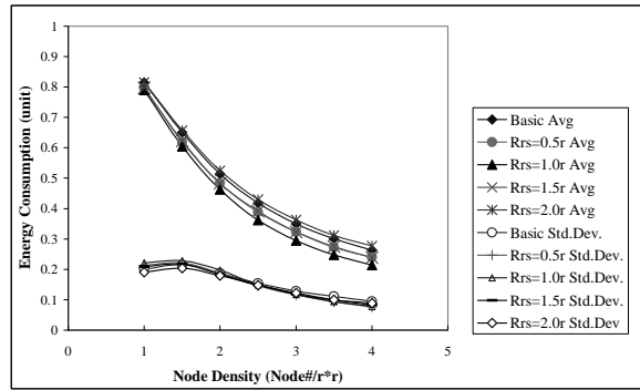
Fig. 27. Total Energy Consumed for Reference Point Scattering
