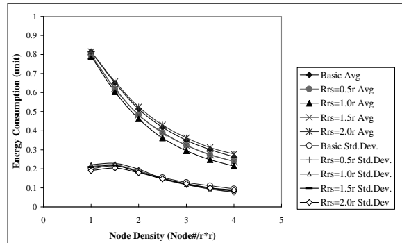
Fig. 27. Total Energy Consumed for Reference Point Scattering
