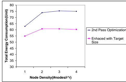
Fig. 21. Total Energy Consumption per Unit of Time(Target Size=2)
