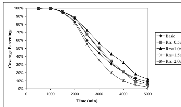
Fig. 29. Coverage Over Time for Reference Point Scattering
