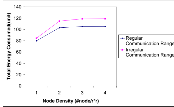
Fig. 35. Total Energy Consumption per Unit of Time
