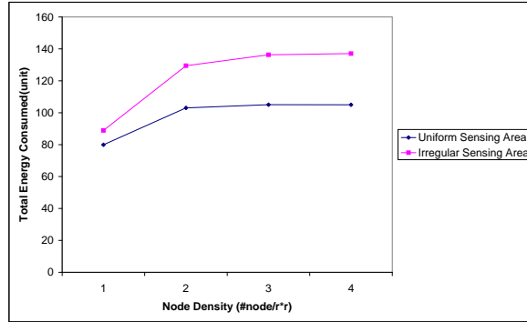
Fig. 33. Total Energy Consumption per Unit of Time
