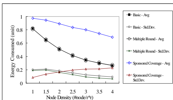
Fig. 12. Single Node Energy Consumption: Average and Standard Deviation
