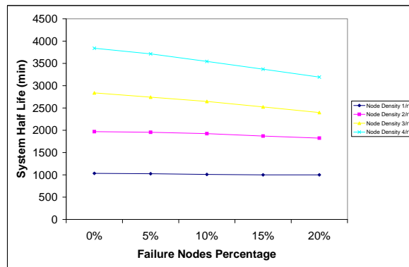
Fig. 37. Half-Life of the Network
