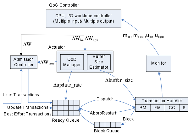
Figure 2: Feedback control architecture
