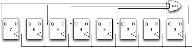
Fig. 1. An 8-bit LFSR with taps at bits 2, 4, 5 and 7. The least significant, or most recently generated, bit is numbered 0. A LFSR with maximum period always has an even number of taps; the oldest bit is always tapped.
