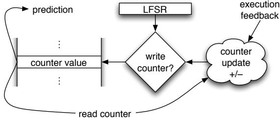
Fig. 2. Probabilistic, LFSR-mediated counter updates.
