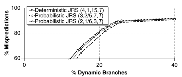
Fig. 7. Probabilistic branch confidence counters have the same behavior as deterministic counters but require less storage.
