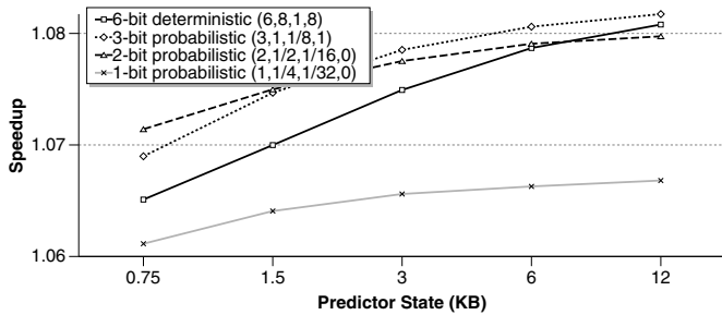
Fig. 6. Speedups for predictors of varying sizes. The 3-bit deterministic predictor (not shown) always offers less than 6% speedup.
