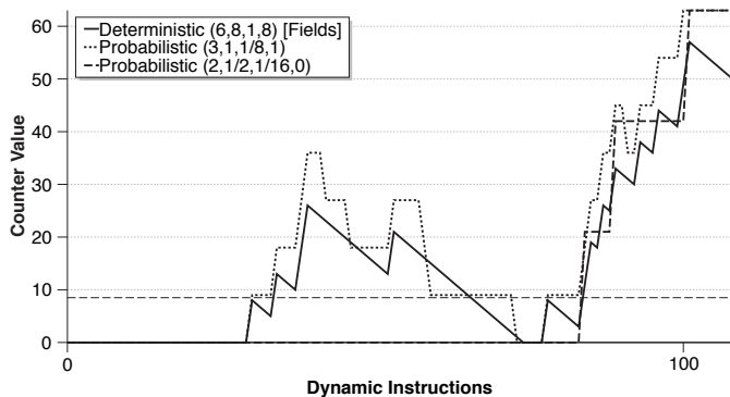
Fig. 4. Comparing values of Fields’s deterministic and two approximating probabilistic counters when predicting model-based criticality of a single static instruction over a partial execution of crafty . The horizontal dashed line indicates the threshold of Fields’s counter; the probabilistic counter values are scaled such that their thresholds are equivalent.
