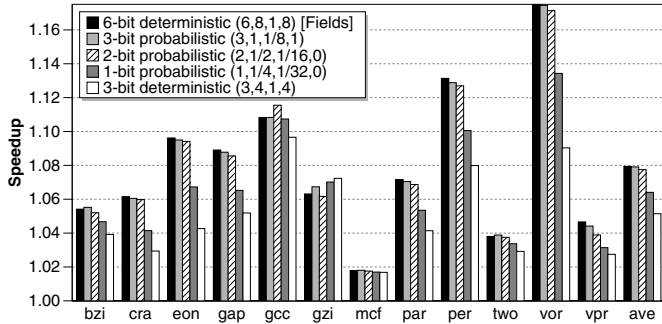
Fig. 5. Speedups over a clustered microarchitecture without critical scheduling, using predictions from model-based criticality results.
