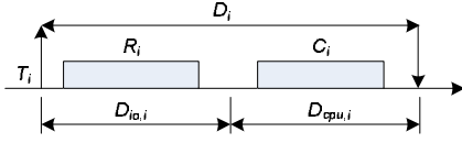
Figure 1: The timing of a typical transaction.
