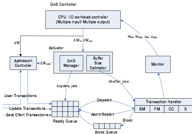
Figure 2: Feedback control architecture
