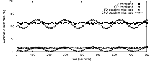
(a) sine wave CPU workload
