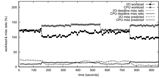
Figure 4: Model validation.
