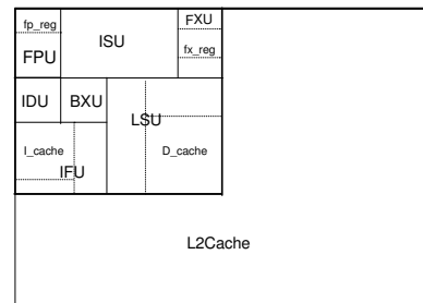
Figure 4: Floorplan used for thermal simulation.
