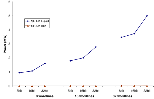
Figure 2: SRAM Power.
