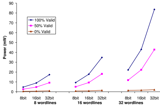
Figure 1: Latch-Mux Power.
