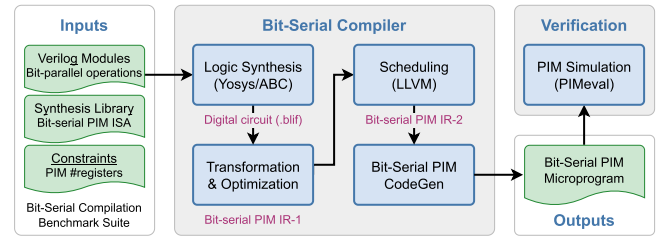
Fig. 3. PIMsynth bit-serial compiler main flow: A unified compilation framework that supports diverse digital and analog bit-serial PIM architectures.
