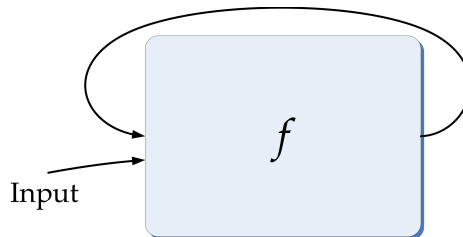
Figure 4.3. Circular Composition.
