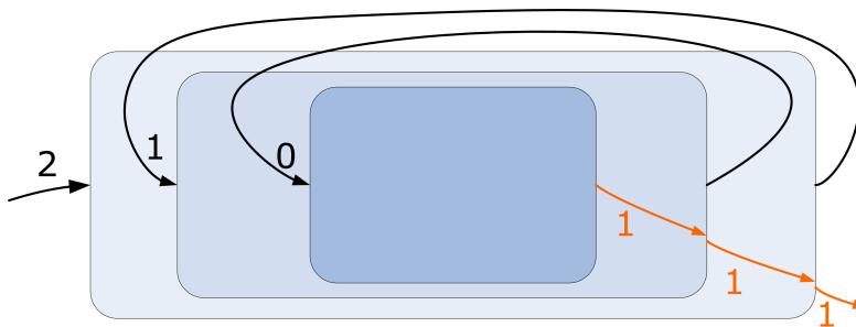
Figure 4.4. Recursive Composition.
