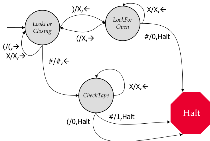
Figure 6.9. Graphical depiction of Turing Machine for checking balanced parentheses.
