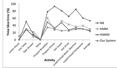
Fig. 4: Comparison of Time Slice Error for Activity Recognition among different classifiers.
