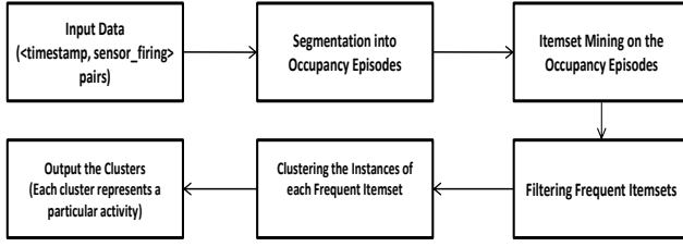
Fig. 1: Block Diagram of the Training Framework
