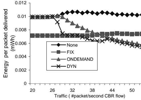
Figure 19: Energy per unit delivered ( one-to-one ).
