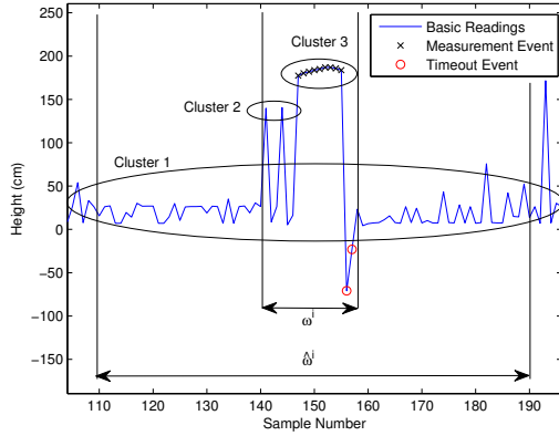
Figure 3. The noise filtering algorithm removes baseline values from window \hat{\omega}_i if they cluster with values from window \omega_i .
