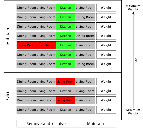
Figure 7. The MHT is composed of many tracks (rows). These are sorted according to their weights and a portion are evicted. The third column is resolved when all tracks agree on the event assignment. Tracks are resolved by removing all preceding state and shortening each individual event sequence.
