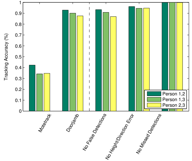
Figure 10. Motetrack achieves 37% tracking accuracy and Doorjamb achieves an average of 90% accuracy. Analysis indicates how much results improve when false detections, height/direction error, and missed detections are removed.
