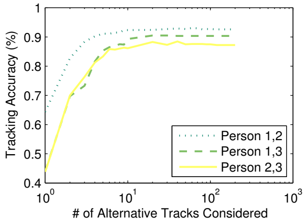
Figure 12. A 4-step path merging algorithm allows Doorjamb to perform well with only 20-30 simultaneous tracks.
