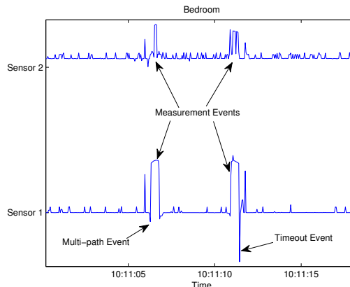
Figure 2. A person in the doorway can cause three different responses from the range finder: (1) Timeout events, (2) Multi-path events, and (3) Measurement events.
