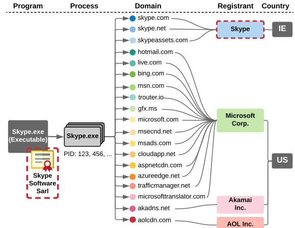
Figure 2: Program-DNS profile of Skype.exe.
