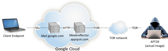
Figure 1: POSHSPY attack injects activities through Windows Management Interface event and leverages Google cloud service to reach its C&C server.
