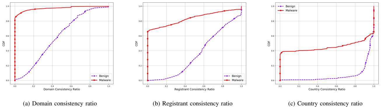
Figure 6: Consistency Ratios for Interactive Processes.
