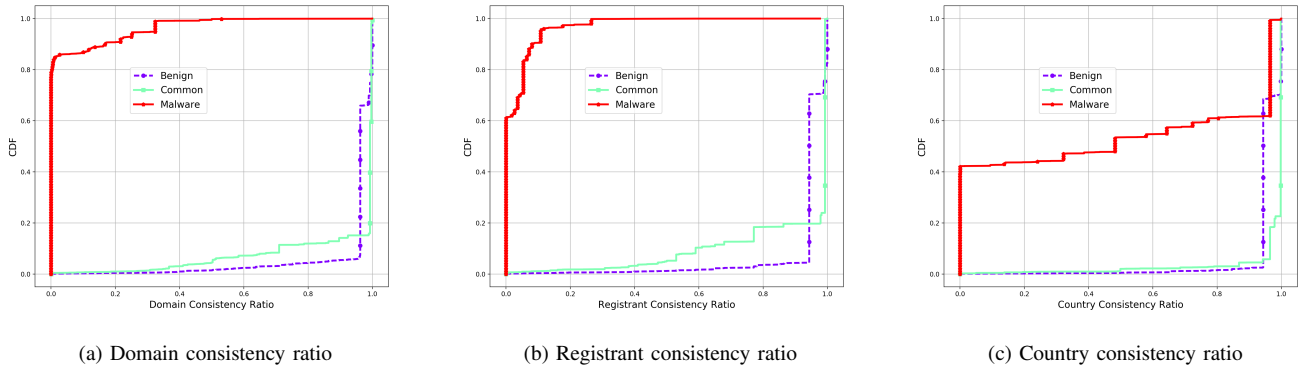
Figure 5: Consistency Ratios for Non-interactive Processes.
