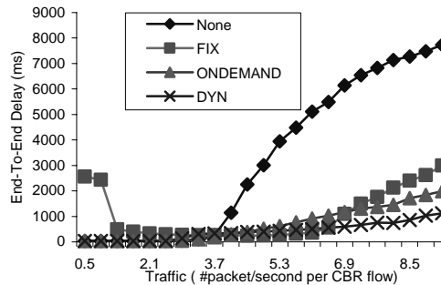
Figure 14: Avg E2E delay (many-to-many 200Kps)
