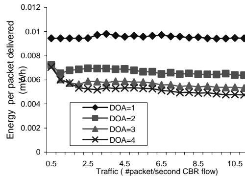
Figure 20: Energy per unit delivered (many-to-one)
