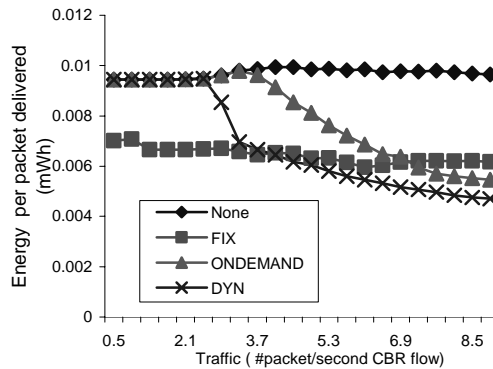
Figure 19: Energy per unit delivered ( one-to-one ).
