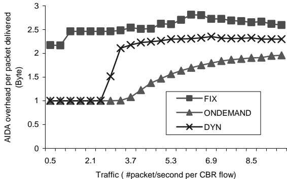
Figure 29: AIDA overhead (one-to-one)
