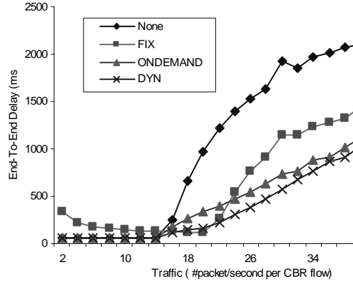
Figure 16: E2E delay (one-to-one under 100Kps)
