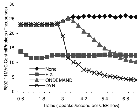
Figure 24: MAC control Packets (many-to-one)
