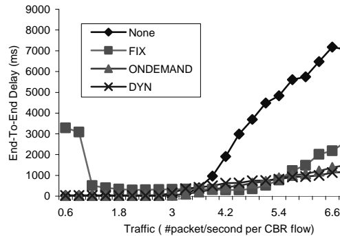
Figure 13: Avg E2E delay (many-to-one 200 Kbps)
