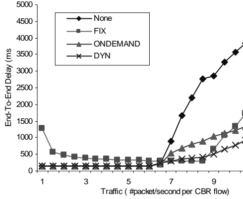
Figure 15: E2E delay (one-to-one under 40Kps)
