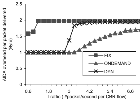
Figure 30: Aida overhead (many-to-one)
