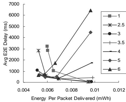
Figure 18 E2E Delay vs. Energy (many to one)
