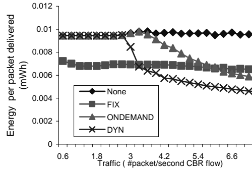
Figure 20: Energy per unit delivered (many-to-one)
