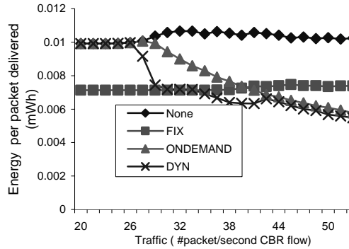
Figure 19: Energy per unit delivered ( one-to-one ).
