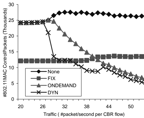
Figure 23: MAC control Packets (one-to-one)
