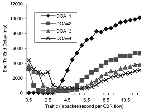
Figure 17: Avg E2E delay (many-to-one)
